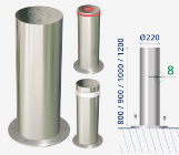
Fixed with base plate Ø220 HP220
